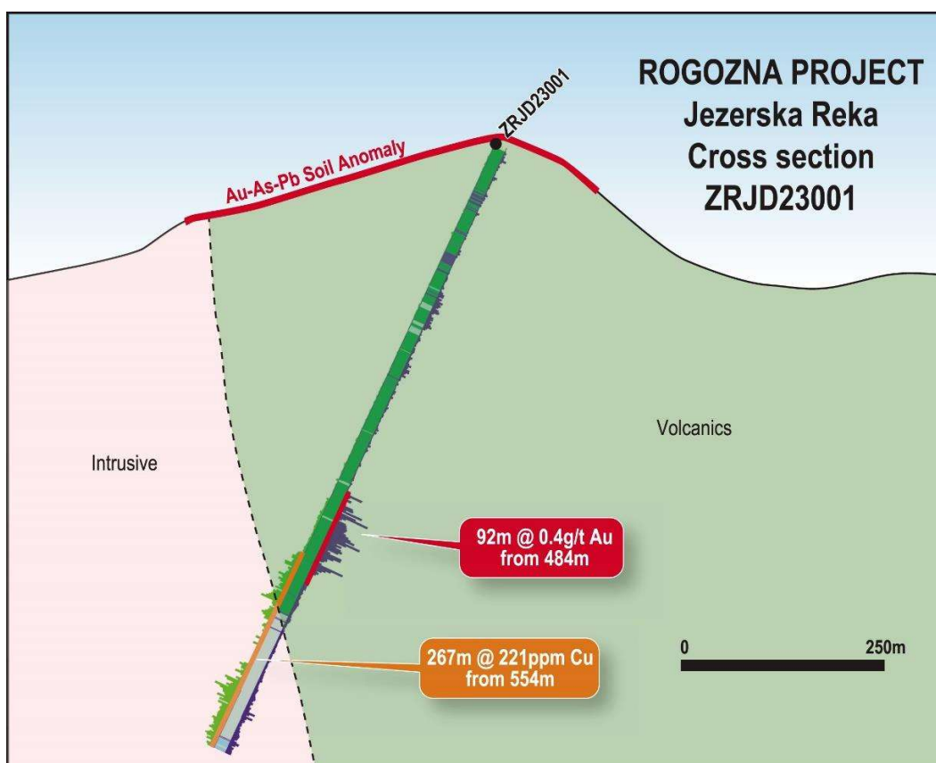
Figure 4. Cross-section view of Jezerska Reka hole ZRJD23001.
