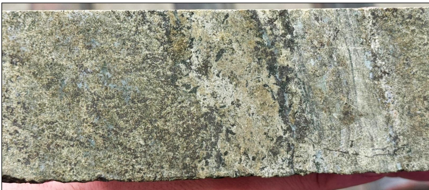
Figure 6. Core photograph of ZRSD25238 from 519.7 to 521.7m of green garnet skarn with disseminated pyrrhotite-pyrite-magnetite-sphalerite-chalcopyrite – 6.3 g/t Au.
