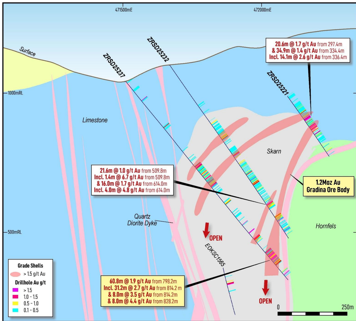
Figure 4. Gradina cross-section view along A-B, showing results for ZRSD25237. 2
